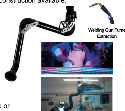
Source Capture Fume Extraction Arm Reach 3' - 40', 5 different diameter sizes. Bench or wall mount, self-supported, easy to position, stainless steel construction available.
